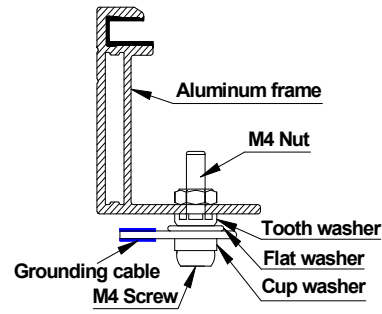
FIG 4 Grounding method
